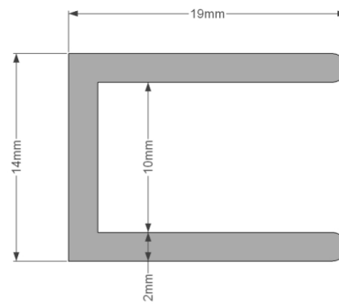
Wall Profile
